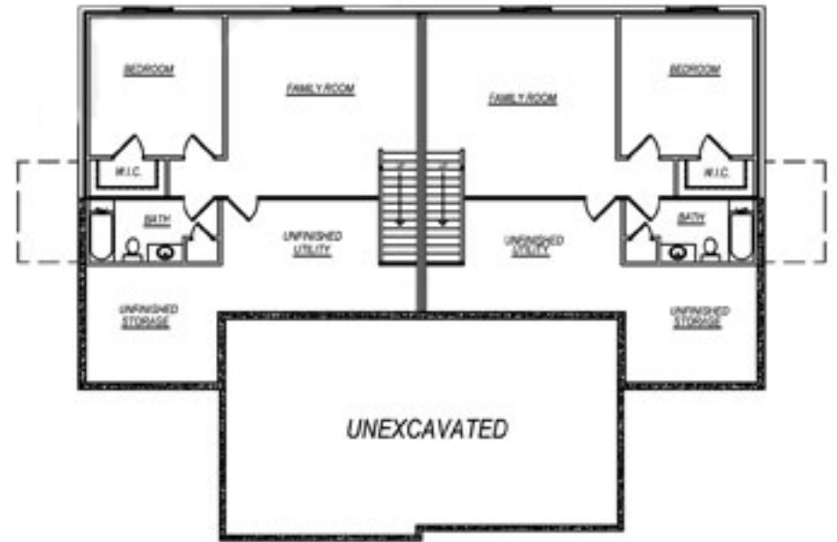
FOUNDATION PLAN
